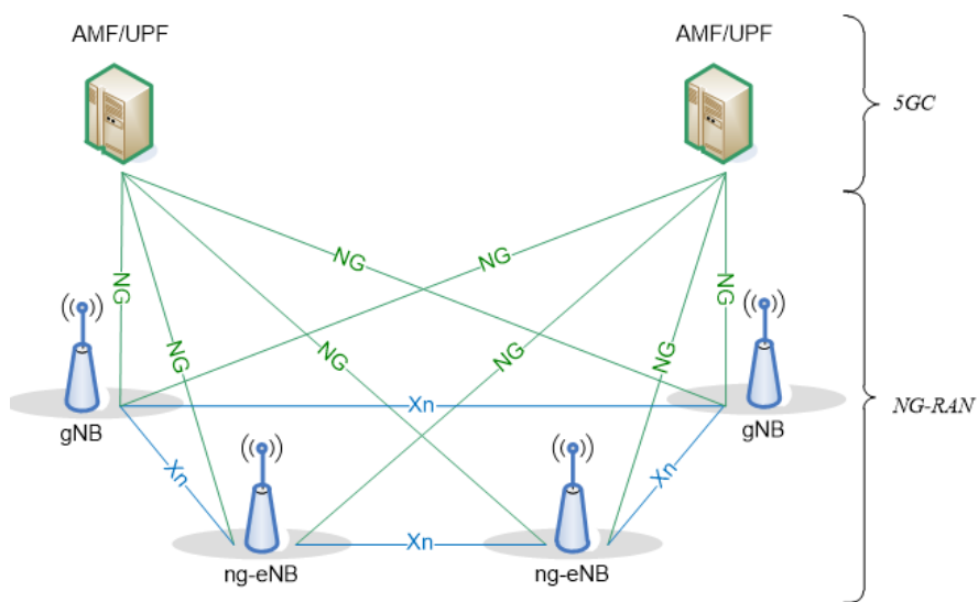
Figure 4.1.2-1: Overall Architecture
