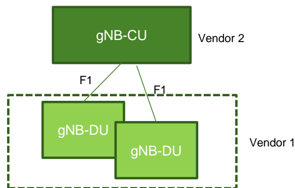
Figure 3.11-3 - CU/DU multi-vendor configuration
