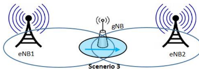
Figure 3.6.2-7 :- Inter MeNB Mobility same SgNB Scenario
