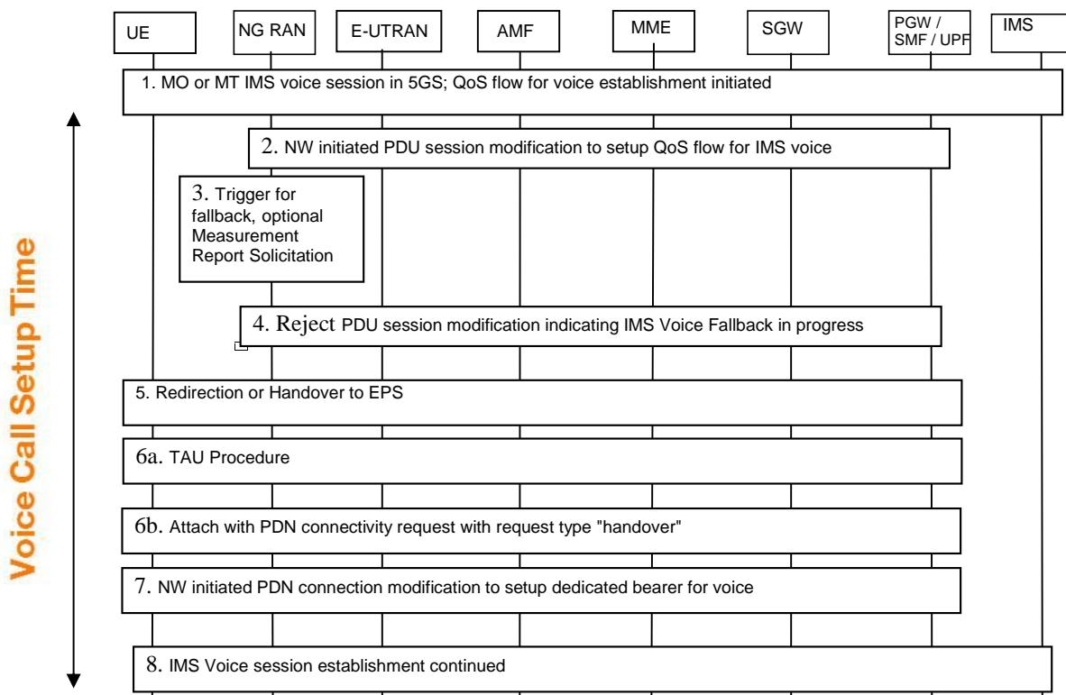
Figure 4.3-1: EPS Fallback for IMS voice
