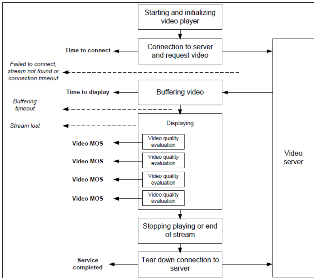
Figure 3.8-2 :- Flow of a typical video service measurement at service level
