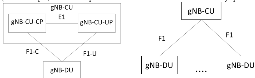
Figure 3.11.2-4 gNB architecture
