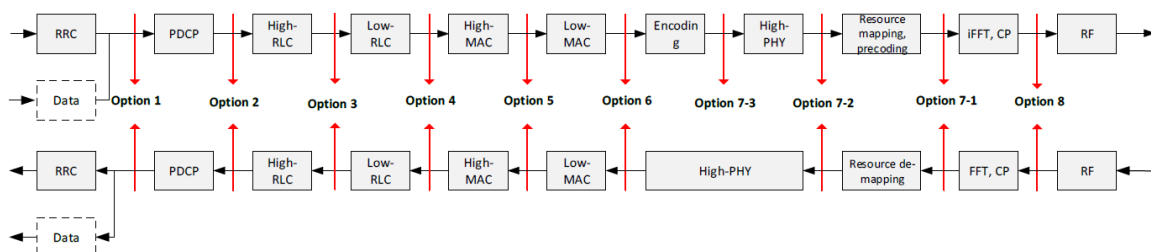
Figure 3.11-1 :- Function Split between central and distributed unit
