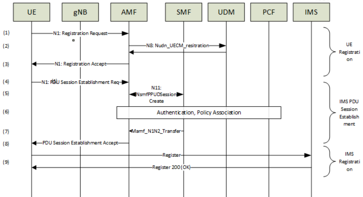
Figure 4.3-2: UE Attach and IMS Registration
