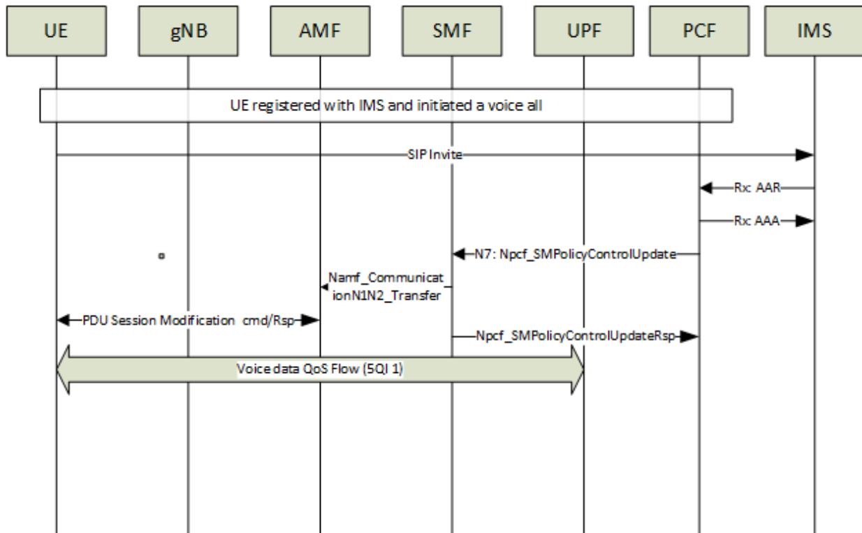
Figure 4.3-3: VoNR call.
