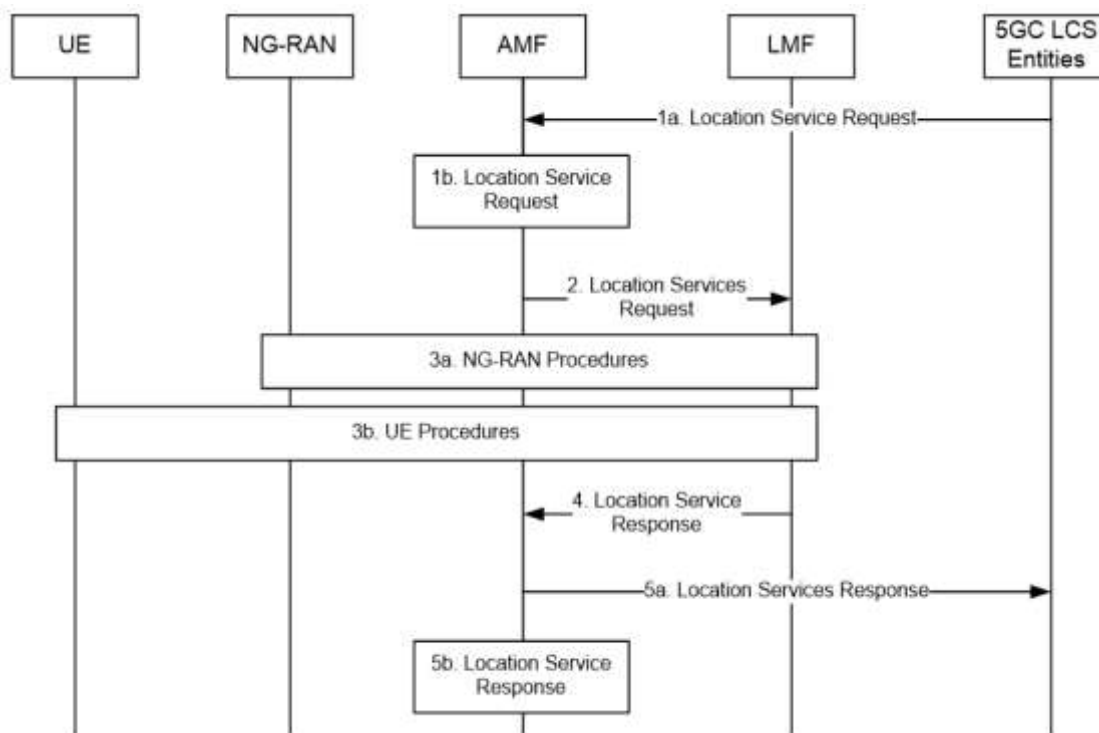
Figure 4.1.2-4: The overall sequence of events applicable to the UE, NG-RAN and LMF for any location service
