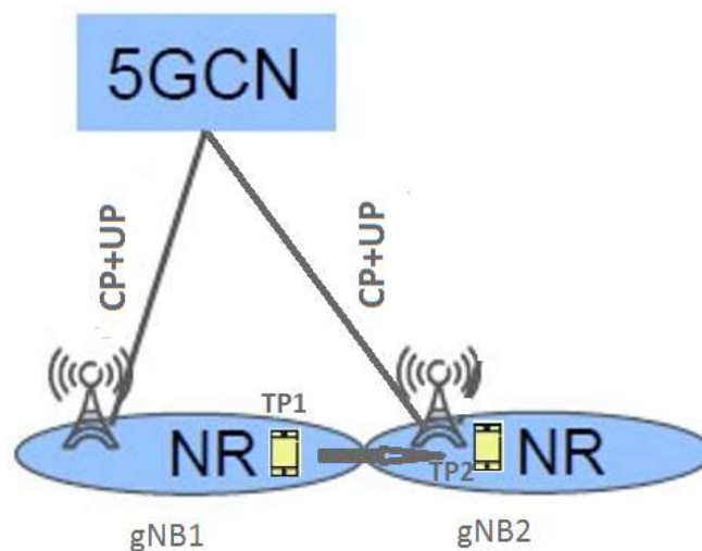
Figure 4.1.2-6 :- Cell Id Test Configuration
