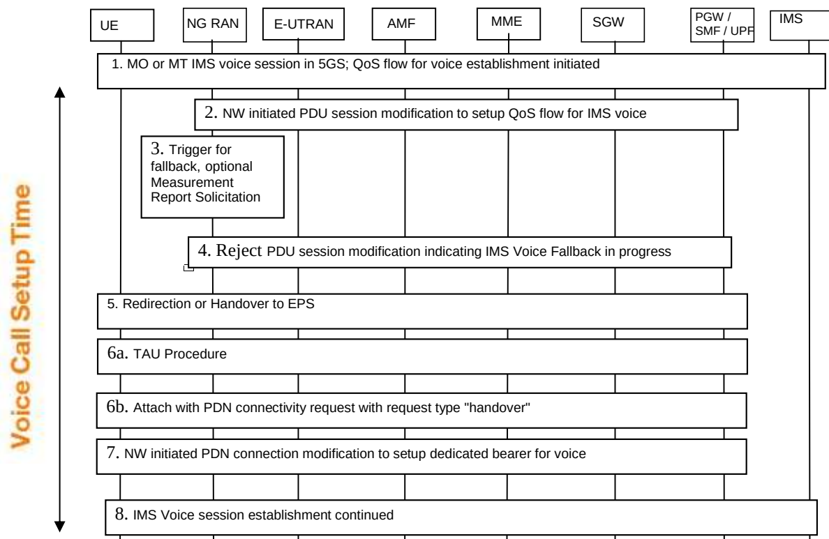
Figure 4.3-1 : EPS Fallback for IMS voice
