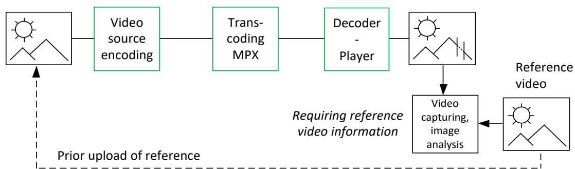
Figure 3.8.2-3 :- Principle of the video flow in streaming quality measurement using a full-reference method
