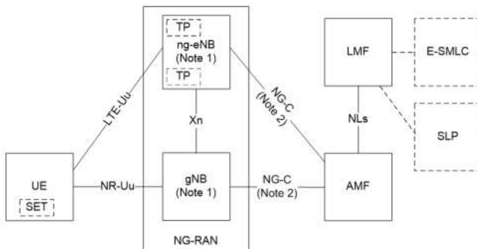
Figure 4.1.2-2: UE Positioning Architecture applicable to NG-RAN
