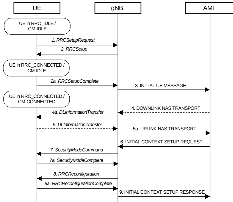
Fig. 3.1.1-3 UE triggered NR RRC Idle to NR RRC Connected transition message flow in SA configuration. (Source: 3GPP TS 38.300 V15.3.1.)
