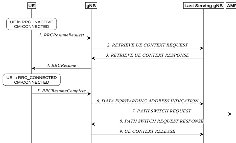
Fig. 3.1.1-4 UE triggered transition from NR RRC_INACTIVE to NR RRC_CONNECTED in SA configuration - UE context retrieval success. (Source: 3GPP TS 38.300 V15.3.1)
