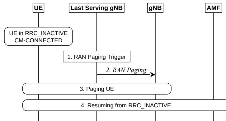
Fig. 3.1.1-5 Network triggered transition from RRC_INACTIVE to RRC_CONNECTED message flow in SA configuration. (Source: 3GPP TS 38.300 V15.3.1)
