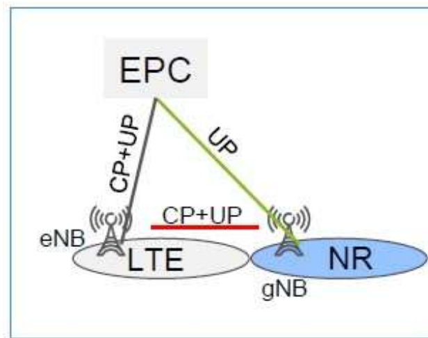
Figure 4.1.1-1 :- Network configuration
