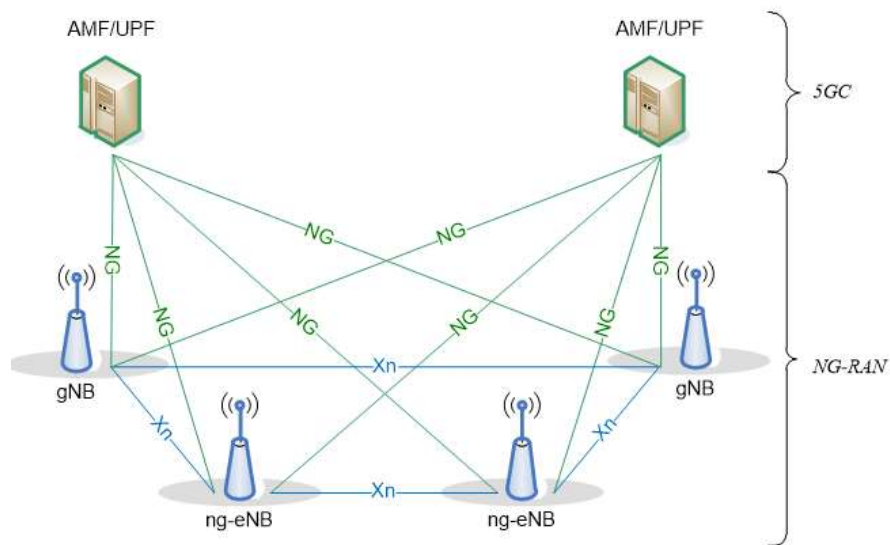
Figure 4.1.2-1: Overall Architecture
