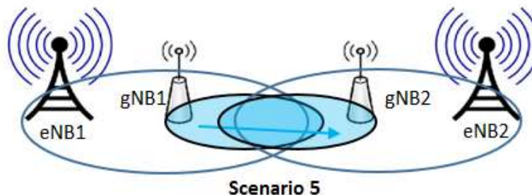
Figure 3.6.2-9 :- Inter MeNB Mobility different SgNB Scenario
