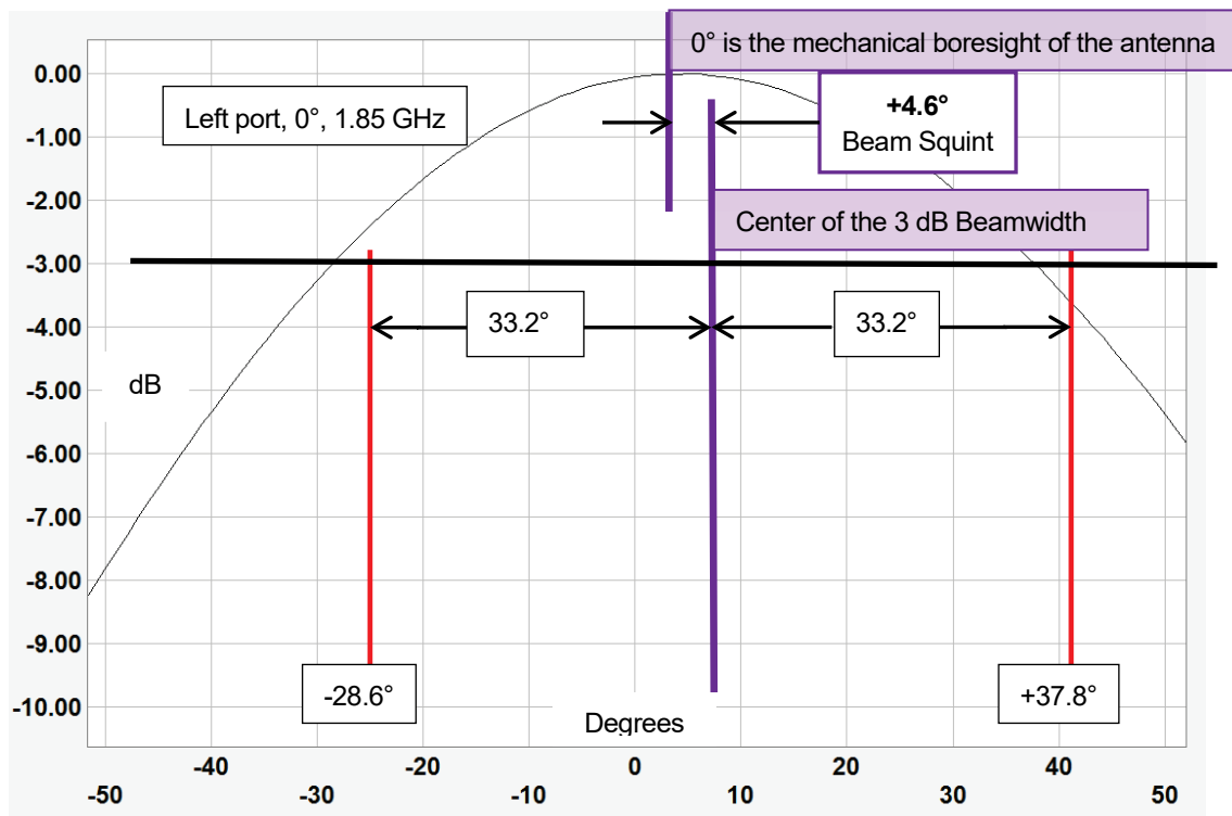
Figure 19—Illustration of beam squint calculation for a given frequency, tilt and port.
