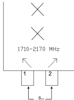
Figure 9—Cross-polar isolation example: single cluster antenna.
