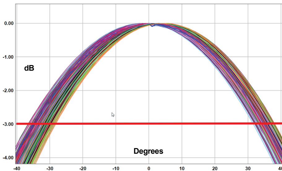
Figure 33—Azimuth beam-peak patterns plots - 1710-1880 MHz, all ports, and all tilts.
