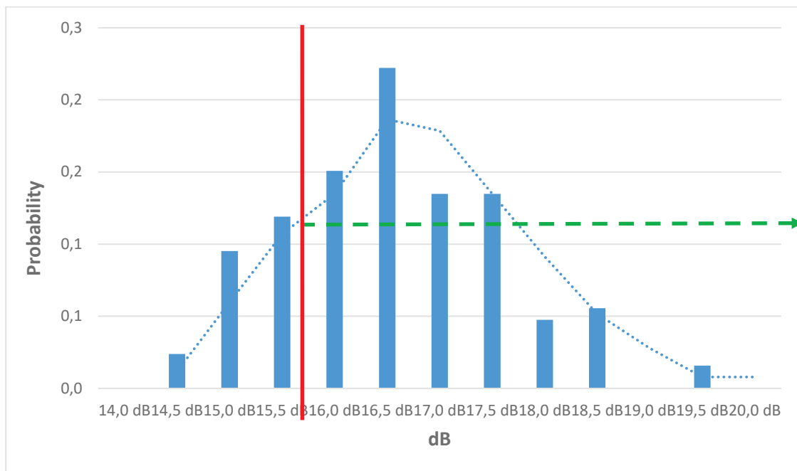
Figure 43—Histogram Upper sidelobe suppression, peak to 20°.
