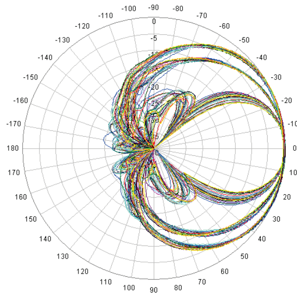
Figure 30— Patterns of a variable azimuth beamwidth BSA (35°/65°/105° pattern overlays).
