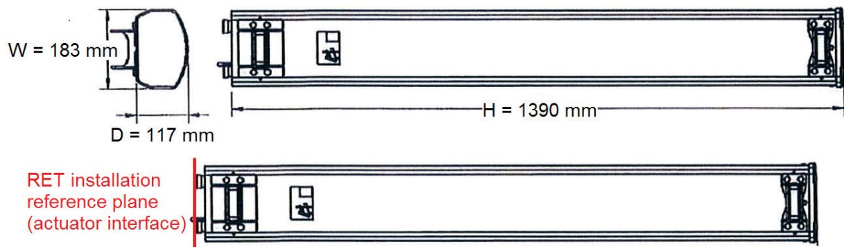
Figure 52—Antenna dimensions example.
