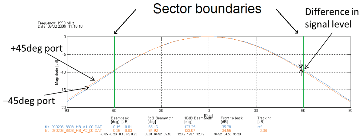
Figure 24—Azimuth beam port-to-port tracking.
