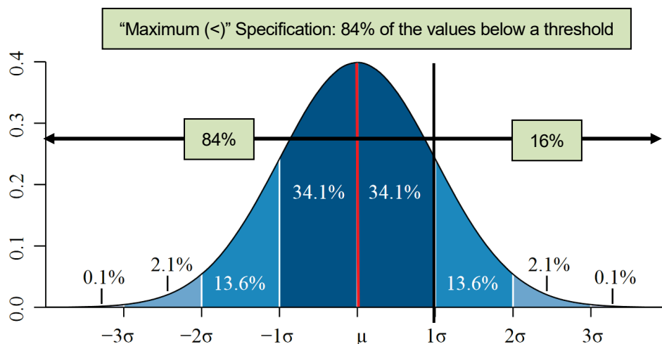
Figure 36—Single-sided specification (maximum).
