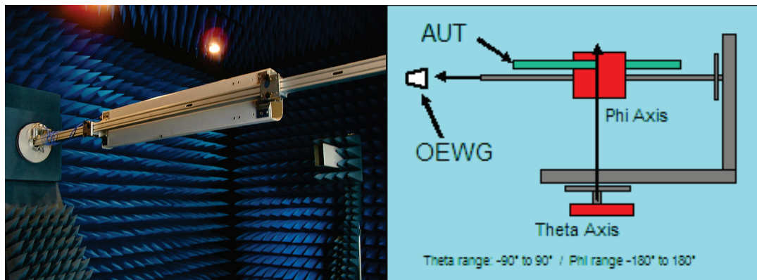
Figure 57—Spherical near-field system.
