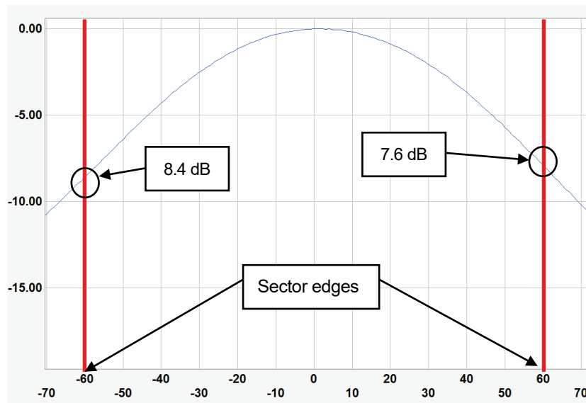
Figure 26—Azimuth beam roll-off.
