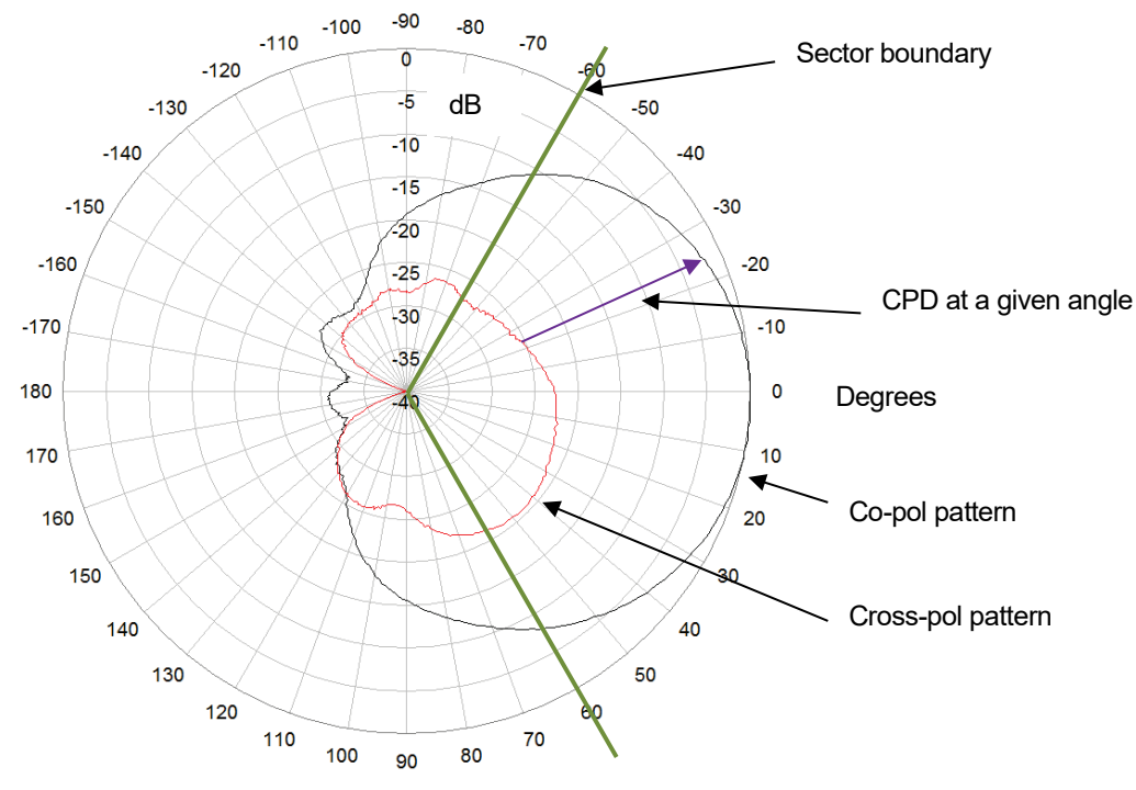
Figure 15—Cross-polar discrimination over sector of a 0° mechanical boresight, 60° nominal horizontal HPBW antenna.
