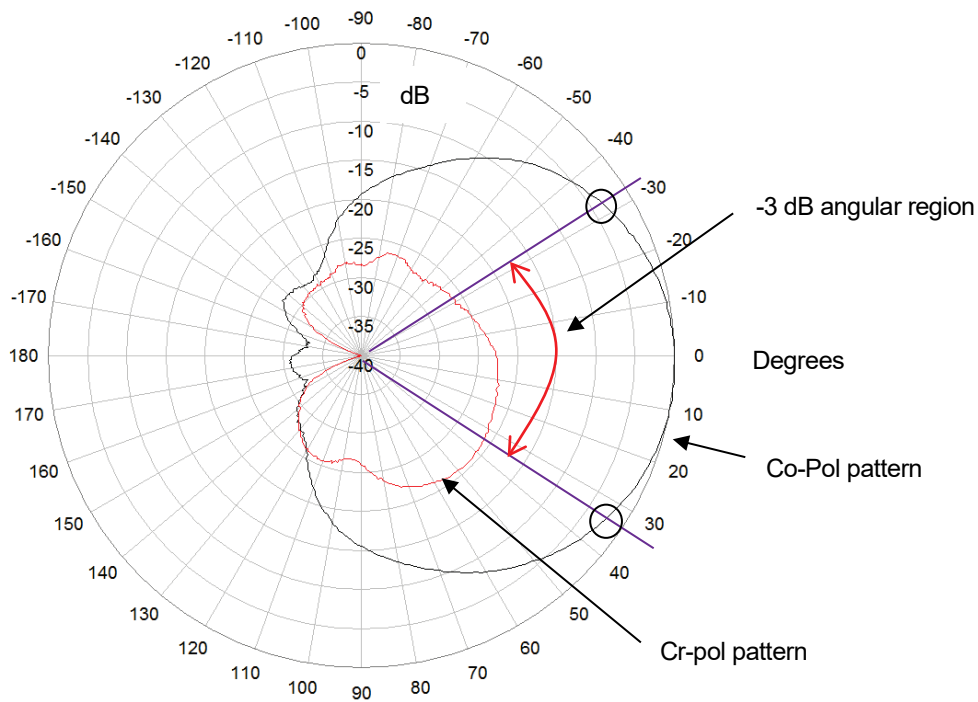
Figure 22—Cross pol discrimination over 3 dB azimuth beamwidth.
