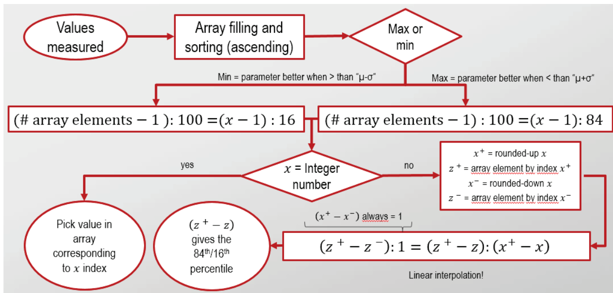
Figure 38—Algorithm to find "maximum" and "minimum".
