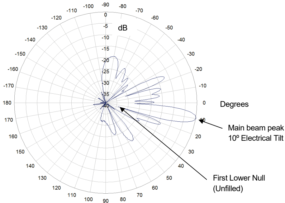
Figure 20—Identification of the lower first null.
