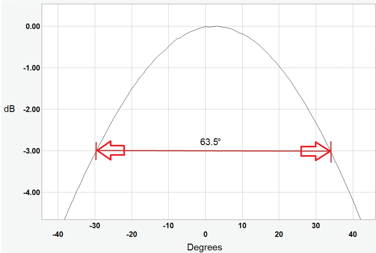
Figure 6—Calculation of azimuth beamwidth.
