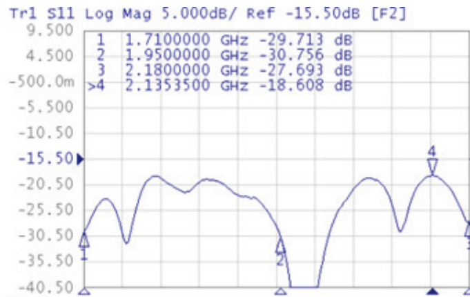
Figure 8—Example of a return loss measurement on a single antenna port.
