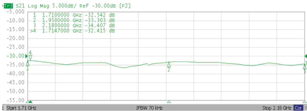
Figure 11—Example of a cross-polar isolation measurement between two antenna ports.
