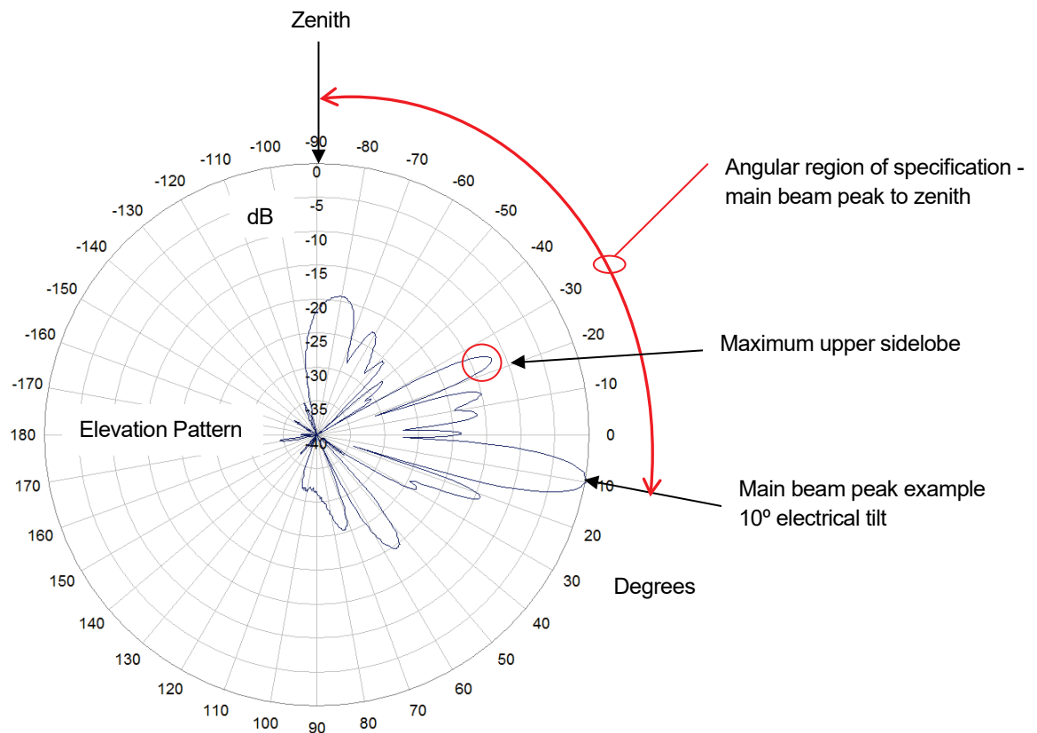
Figure 28—Maximum Upper Sidelobe Level.
