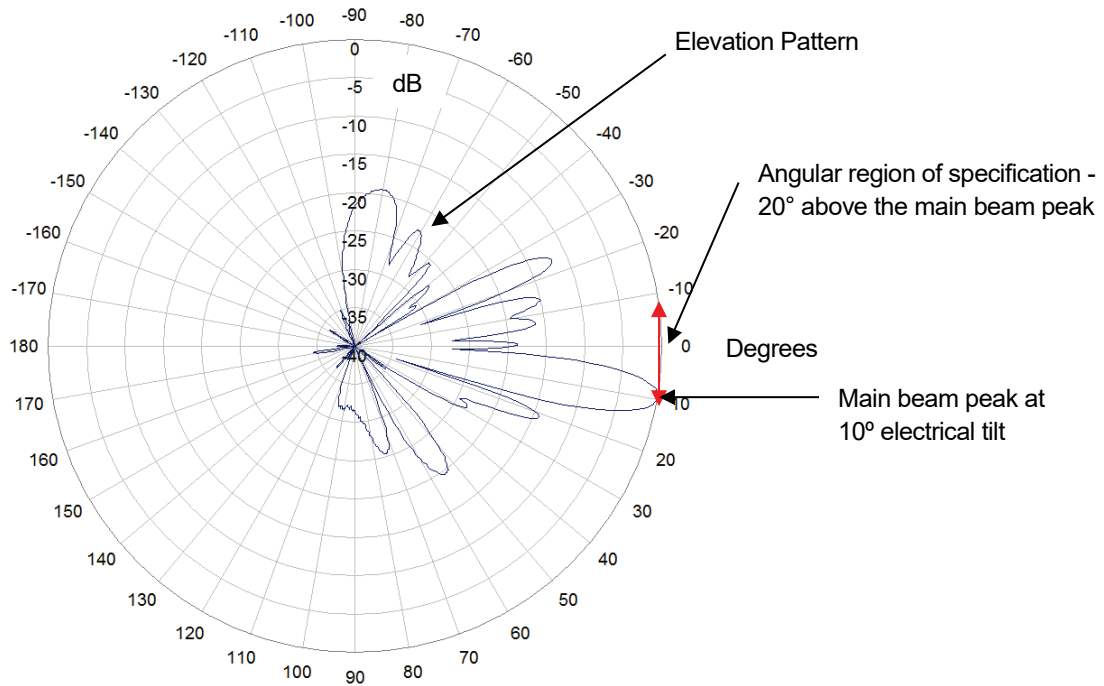
Figure 14—Upper sidelobe suppression, peak to 20°.
