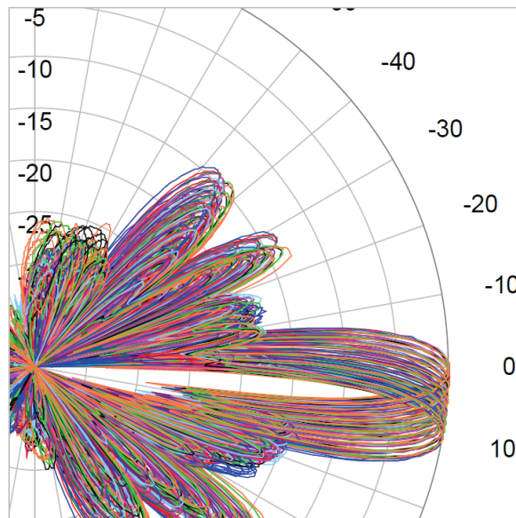
Figure 51—Elevation pattern plots – 1710-1880 MHz, all ports, and all tilts.
