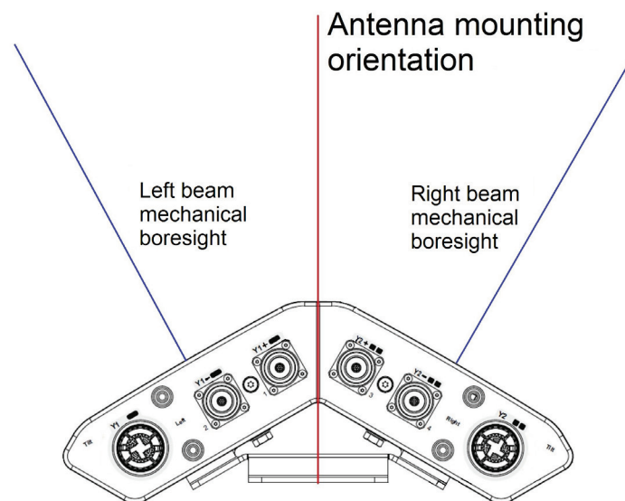
Figure 3—Example of a dual-beam antenna. Its mounting orientation is aligned along 0^\circ . Left and right mechanical boresights are respectively pointed to -30^\circ and +30^\circ .
