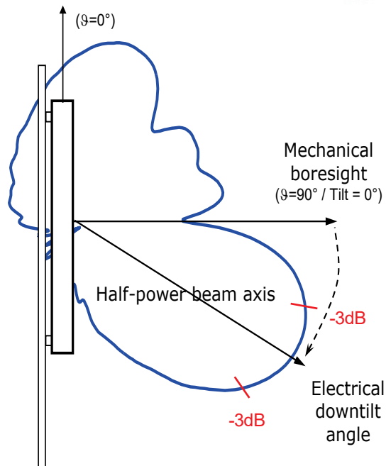
Figure 5—Electrical downtilt angle.
