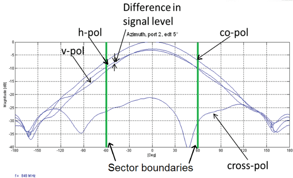
Figure 25—Azimuth beam H/V tracking.
