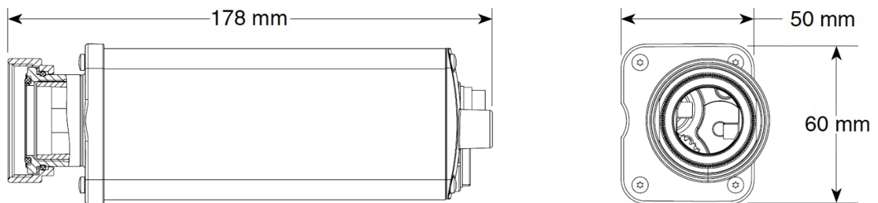
Figure 54—Example of an external RET.
