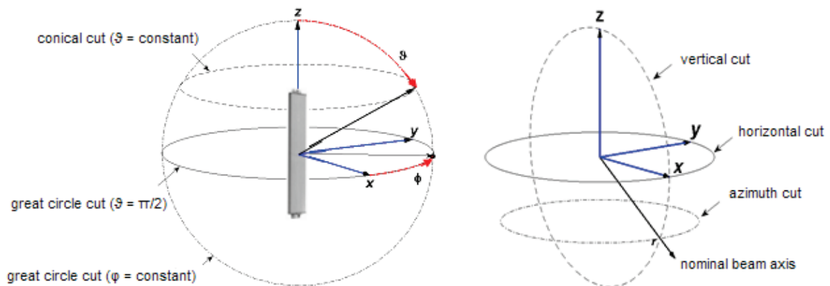
Figure 2—Conical and great circle cuts over the radiation sphere.
