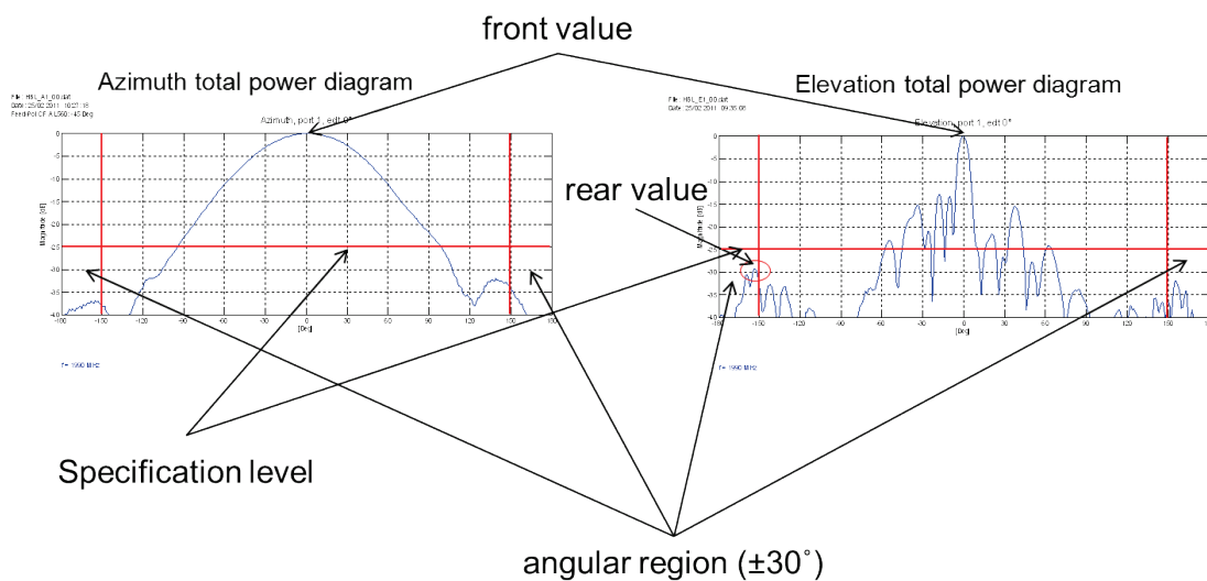
Figure 18—F/B angular regions, azimuth and elevation.
