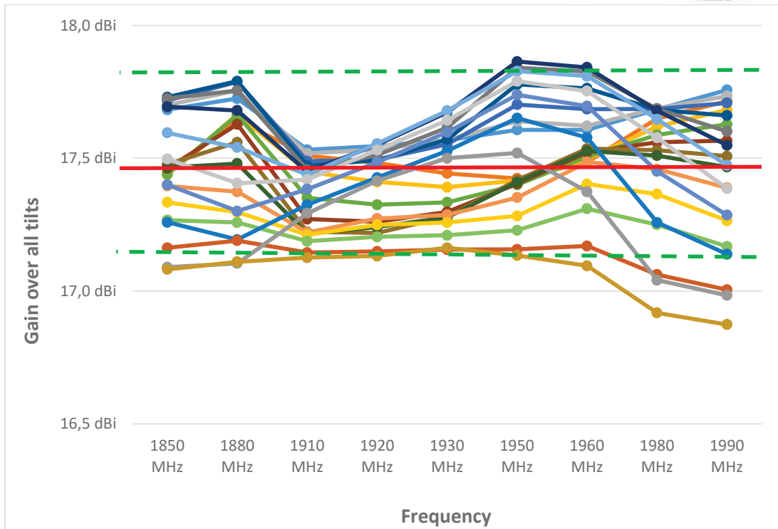
Figure 48—Gain for each tilt and port as a function of the frequency.
