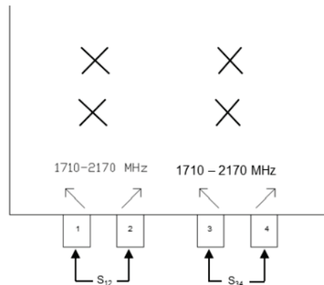
Figure 9—Cross-polar isolation example: single cluster antenna.
