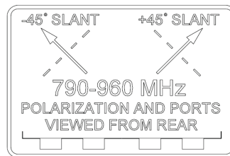
Figure 59—Example of polarization conventional label.
