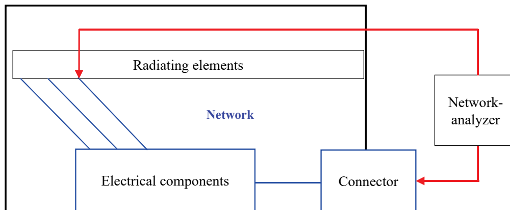
Figure 58—Block diagram of loss measurement.
