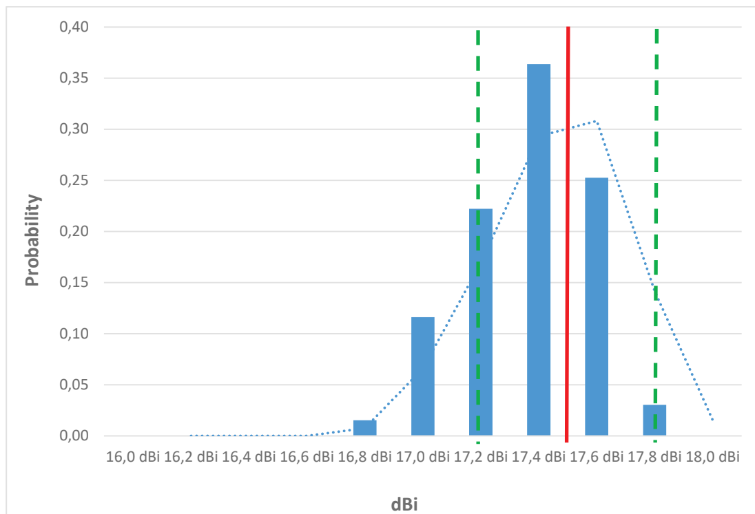
Figure 49—Gain histogram.
