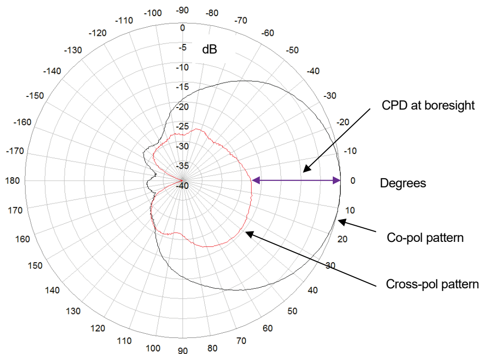
Figure 21—Cross-polar discrimination at mechanical boresight.
