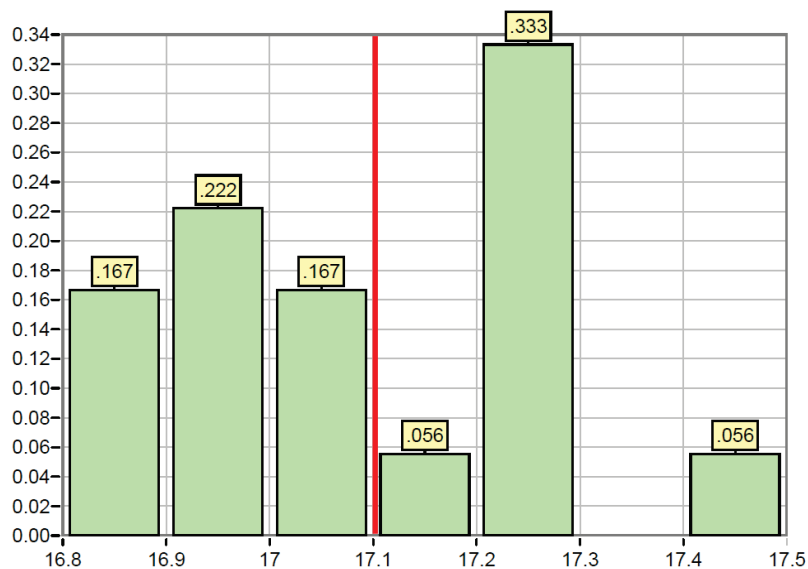
Figure 46—Gain histogram.
