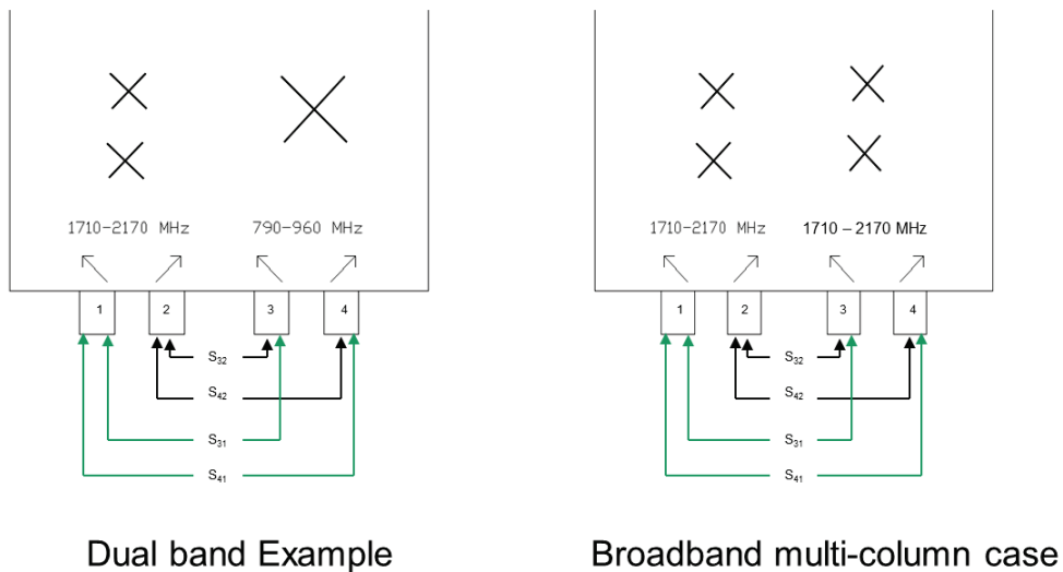
Figure 16—Interband isolation examples. In this example, the interband isolation is the worst case of S41, S31, S42 and S32.
