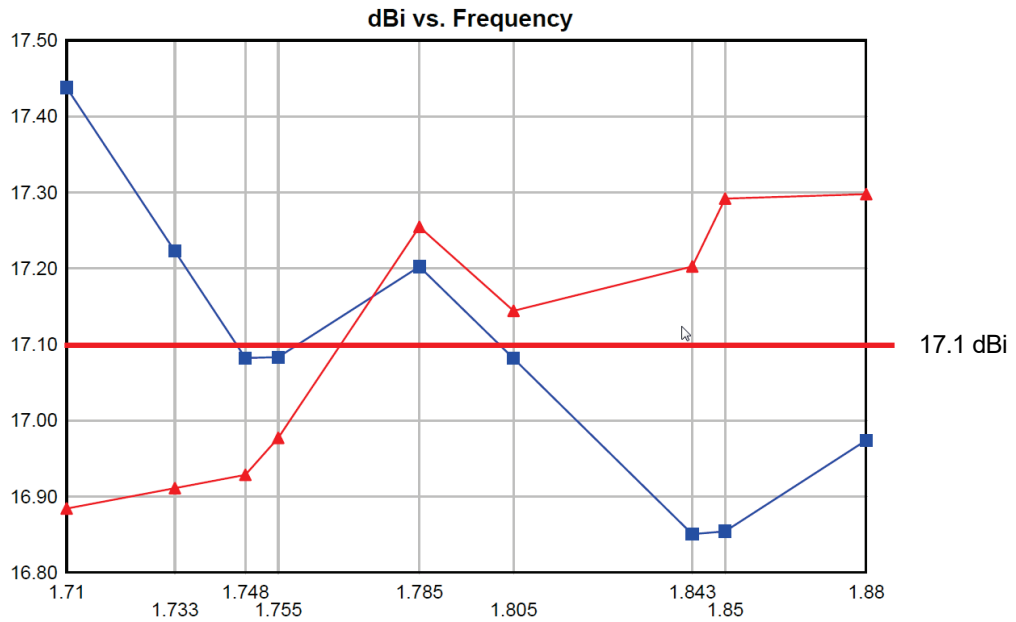
Figure 45—Gain plot for 0° tilt, both ports.
