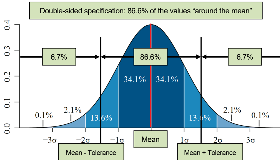
Figure 31—Double-sided specification for a normal distribution.
