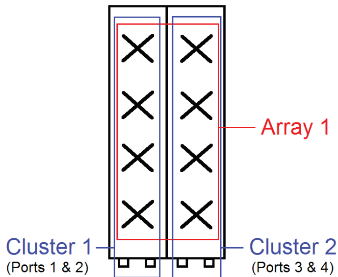
Figure 1—Possible difference between array and clusters.
