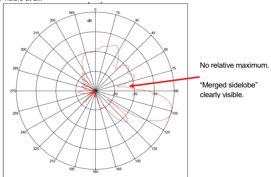
Figure 44—First upper sidelobe merged into main beam.
