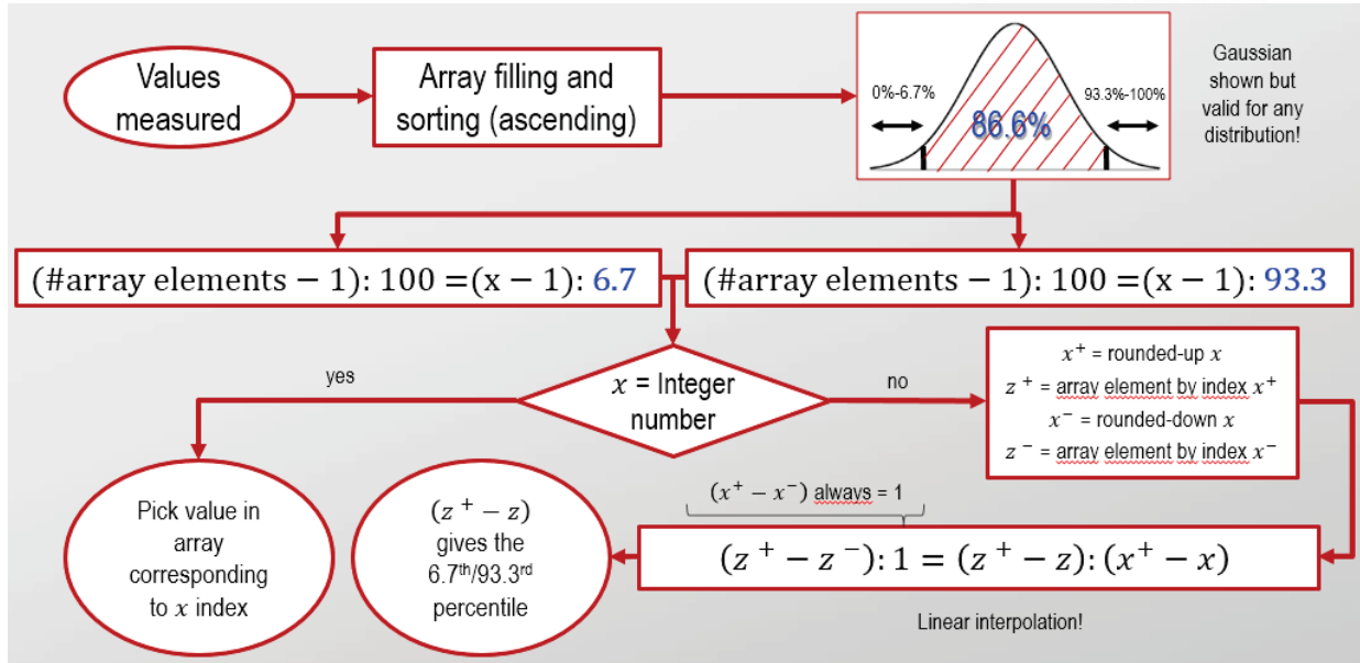
Figure 32—Algorithm to find "mean - tolerance" and "mean + tolerance"
