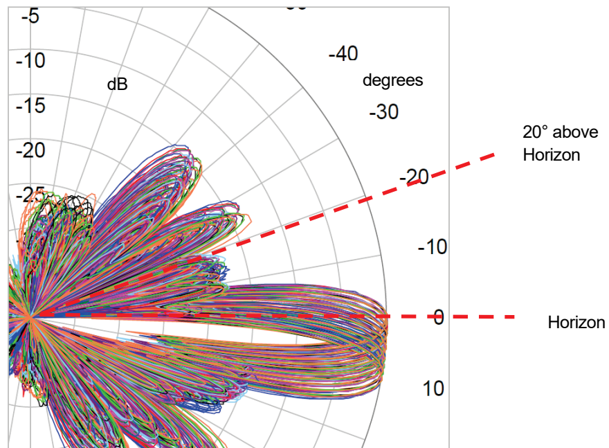
Figure 27—Upper sidelobe suppression, horizon to 20°.
