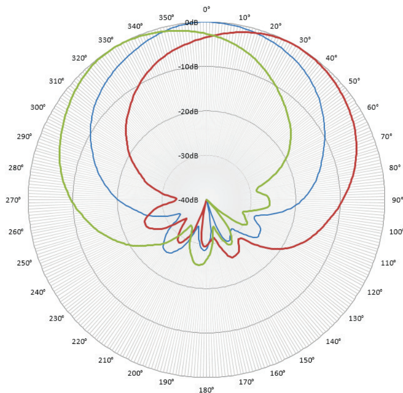
Figure 29—Some patterns of an azimuth beam steering antenna (pan angles: -30°; 0°; +30°).
