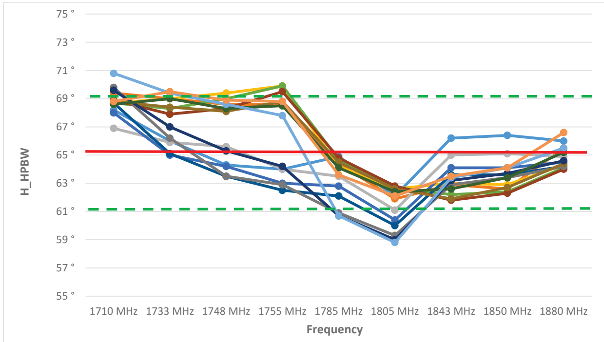
Figure 34—Azimuth HPBW for each tilt and port as a function of the frequency.
