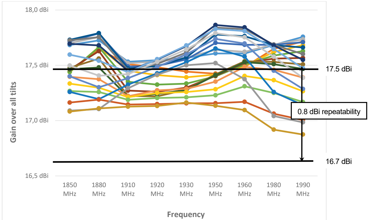
Figure 50—Gain plot with repeatability margin.
