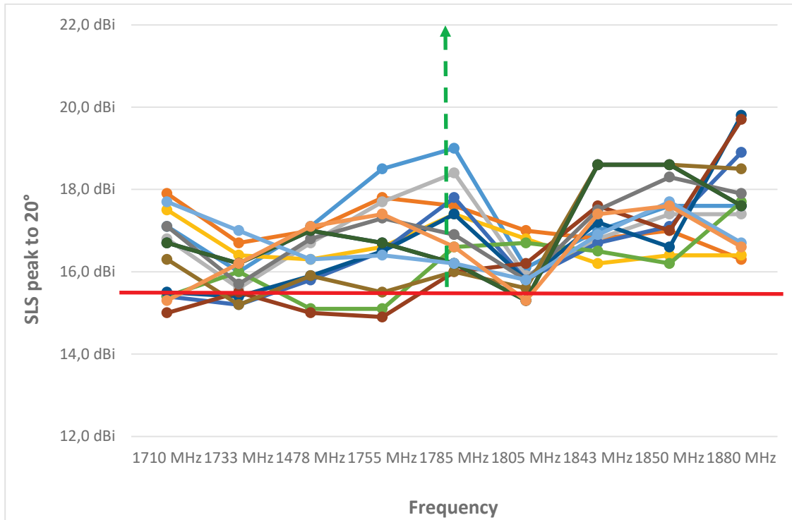
Figure 41—Upper sidelobe suppression, peak to 20° for each tilt and port as a function of the frequency.
