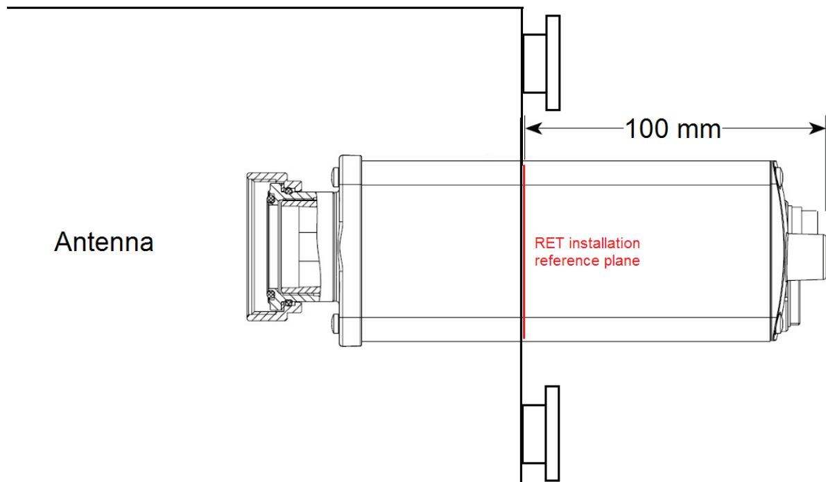
Figure 55—Example of the height dimension of an installed partially external RET. Its protrusion out of the antenna lies along the antenna height plane (H).
