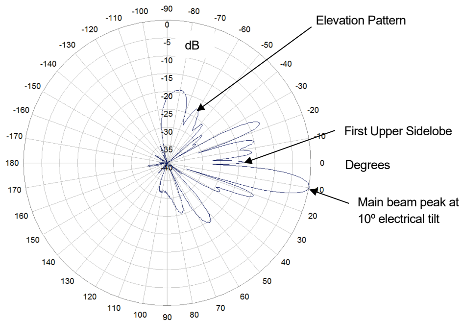
Figure 13—First upper sidelobe suppression.
