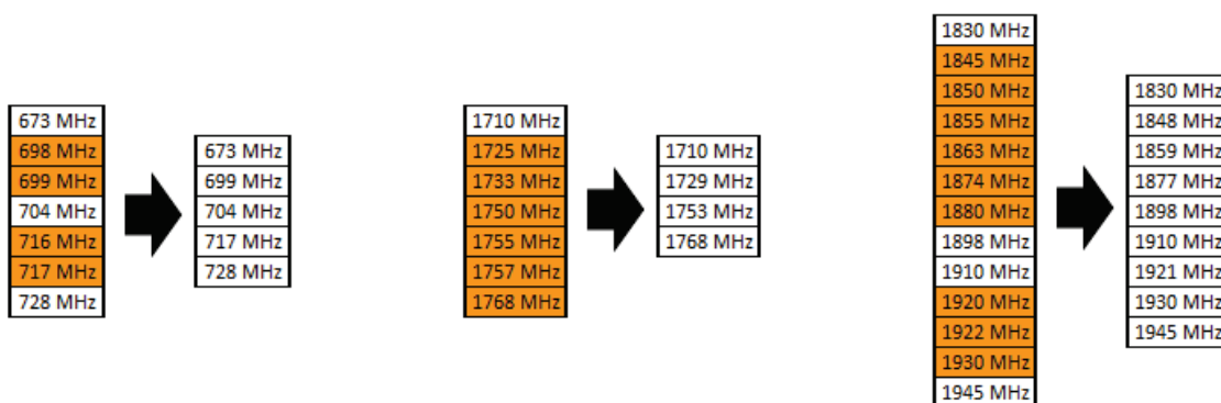
Figure 56—Examples of frequency samples redundancy optimization.
