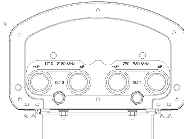
Figure 61—Ports identified by polarization.
