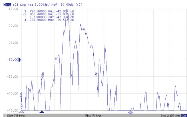
Figure 17—Interband isolation vs. frequency on a single pair of ports.
