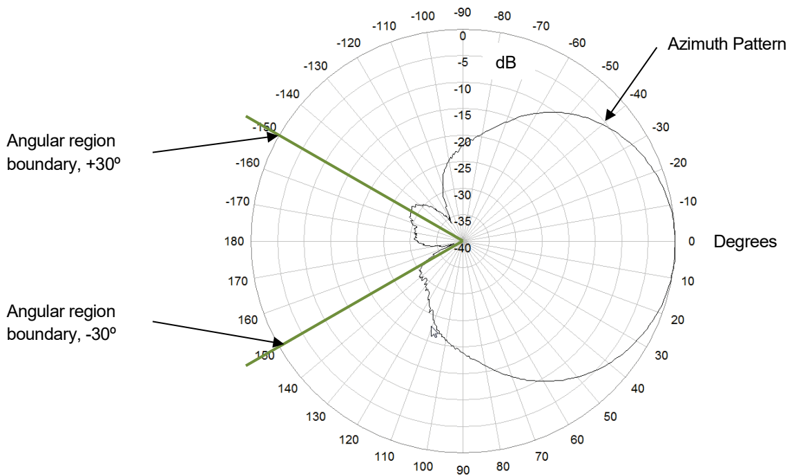
Figure 12—Angular region for front-to-back, total power ± 30° of a 0° mechanical boresight antenna.
