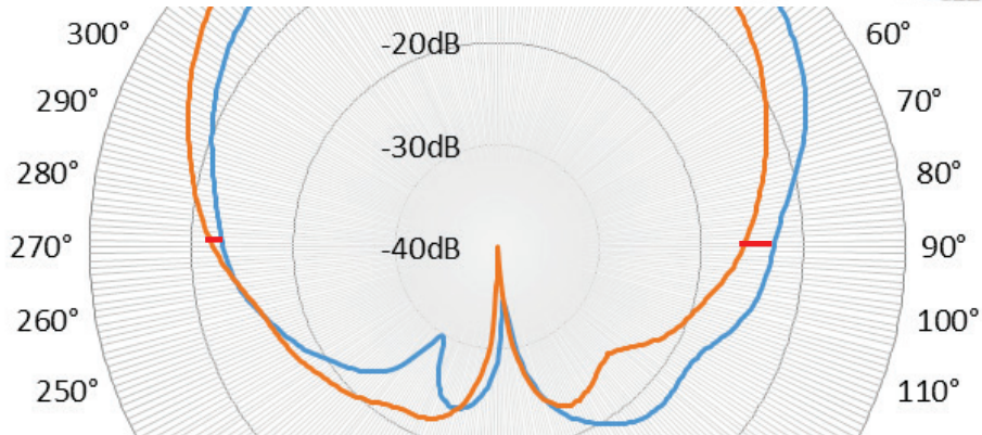
Figure 39—Polarizations pattern level difference of a 90° sector antenna for one frequency and a single downtilt degree.
