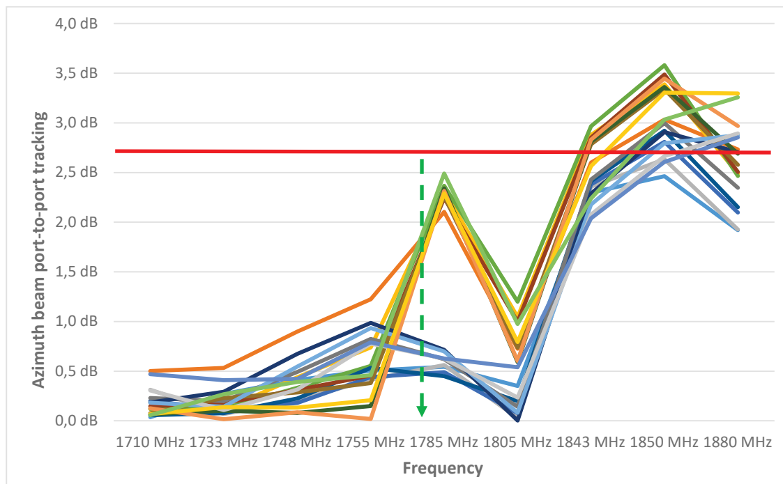
Figure 40—Azimuth beam port-to-port tracking for each tilt and port as a function of the frequency.
