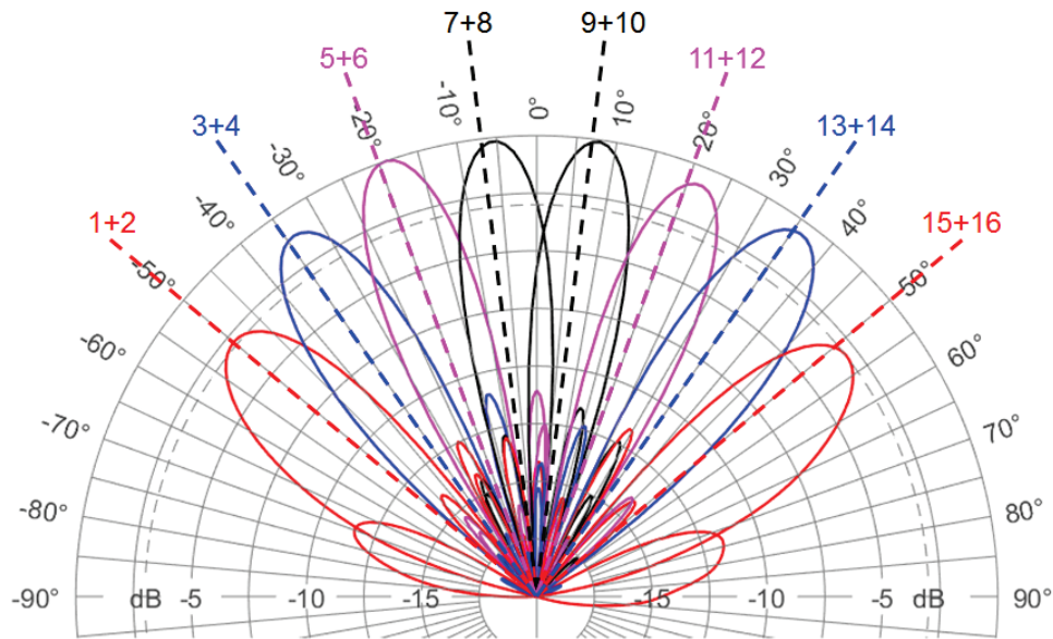
Figure 4—Azimuth pattern of a multi-beam antenna type II. Mounting orientation and mechanical boresight are aligned along 0°. Nominal directions are noted with dotted lines. Each beam is associated to a pair of ports only as a device. All the 16 ports collaborate to produce the pattern shown.
