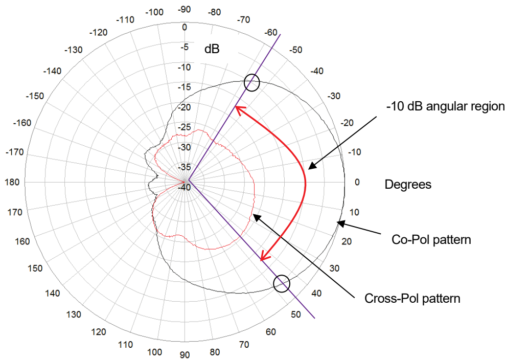
Figure 23—Cross pol discrimination over 10 dB azimuth beamwidth.
