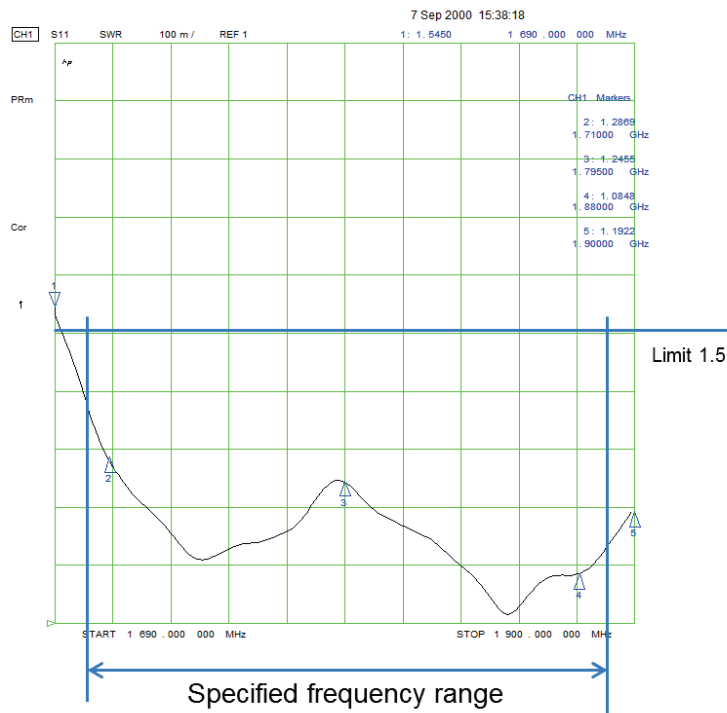
Figure 7—Example of VSWR measurement of an antenna port.
