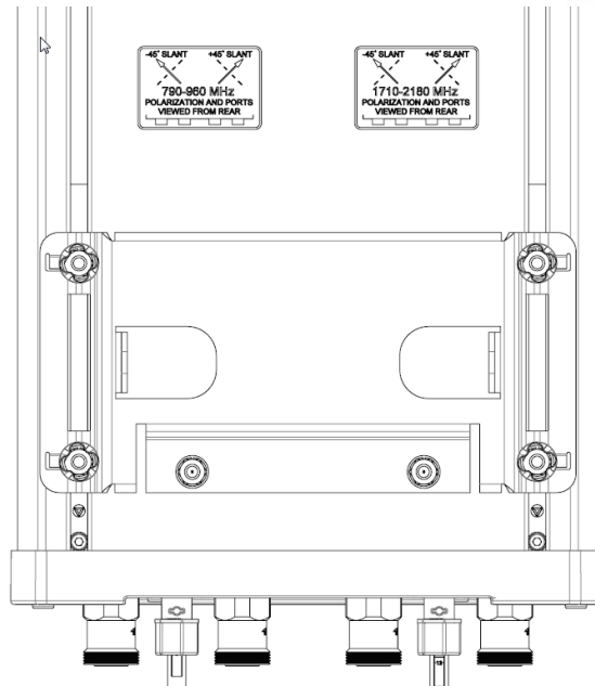
Figure 60—Polarization conventional label affixed on the antenna back.
