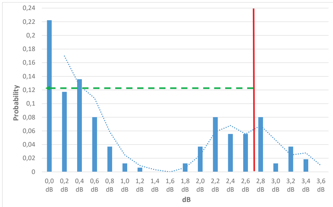
Figure 41—Histogram azimuth beam port-to-port tracking.
