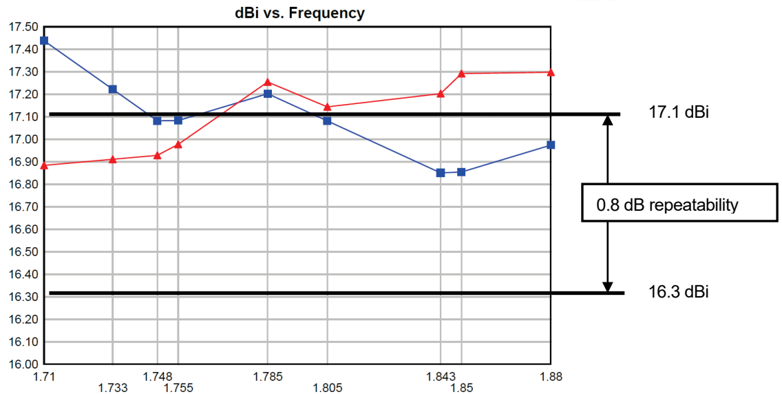
Figure 47—Gain plot with repeatability margin.
