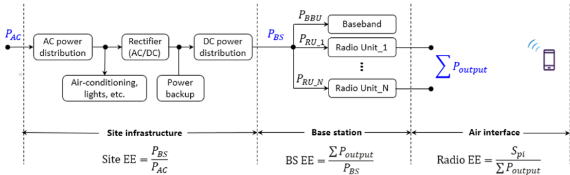
Figure 2: Illustration of a typical RAN site, and energy flow from main AC input to reception at the user terminal.
